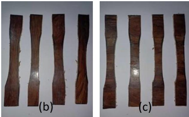
Fig. 4. Gauge (a) Longitudinal (b) and Transverse Fibre (c) Oriented Composite Samples.
