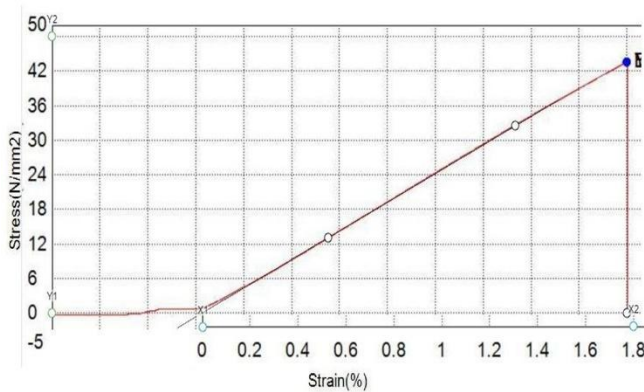
Fig.7. Stress-Strain Diagram of Transverse Fibre Oriented Composite.
