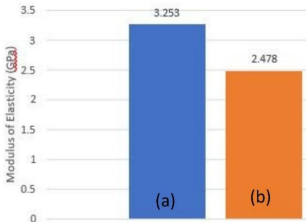
Fig. 8. Maximum Modulus of Elasticity of Longitudinal (a) and Transverse Fibre Oriented Composite.
