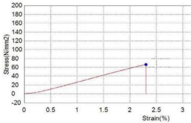
Fig.6. Stress-Strain Diagram of Longitudinal Fibre Oriented Composite.
